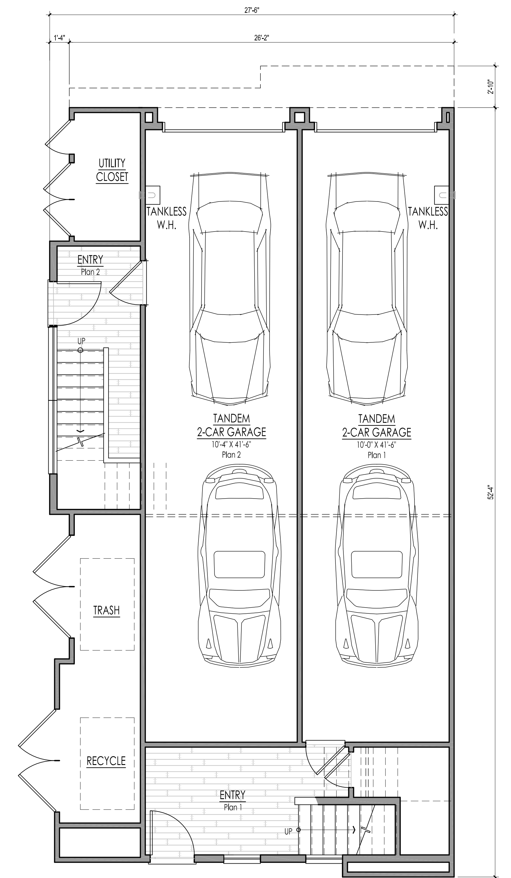
FIRST FLOOR
