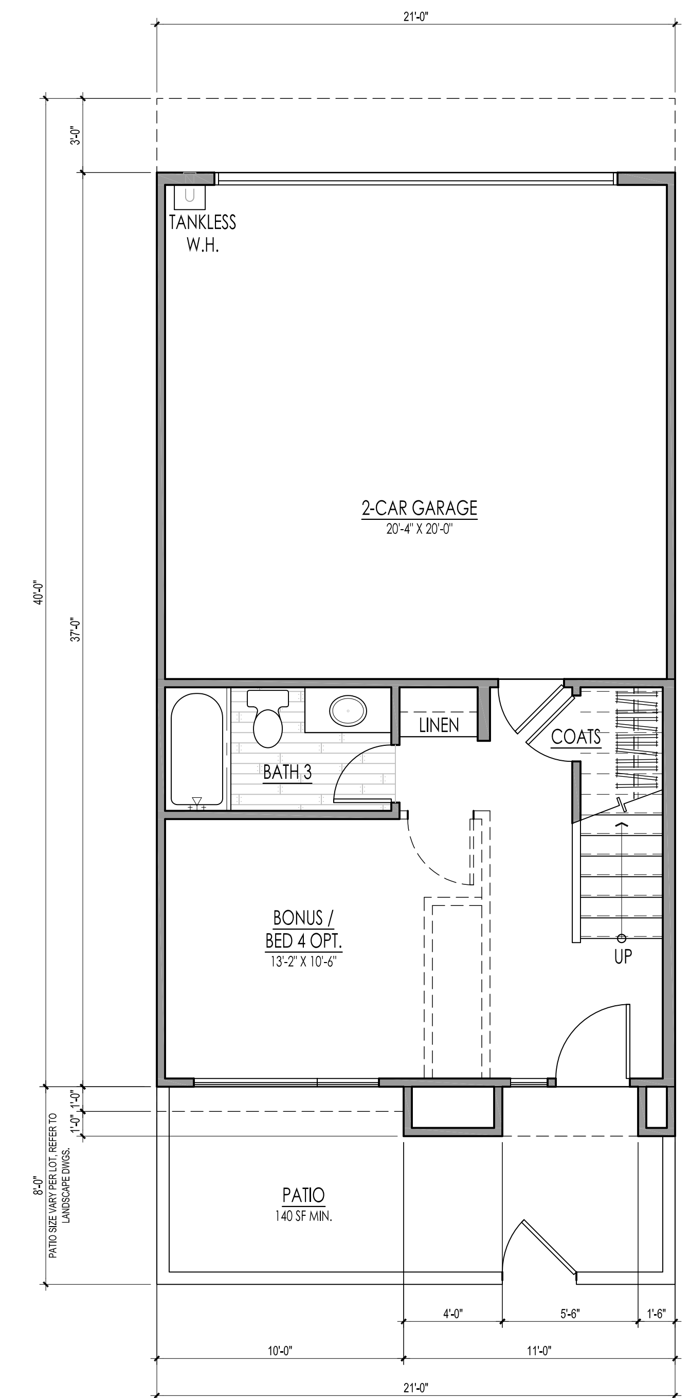
FIRST FLOOR
