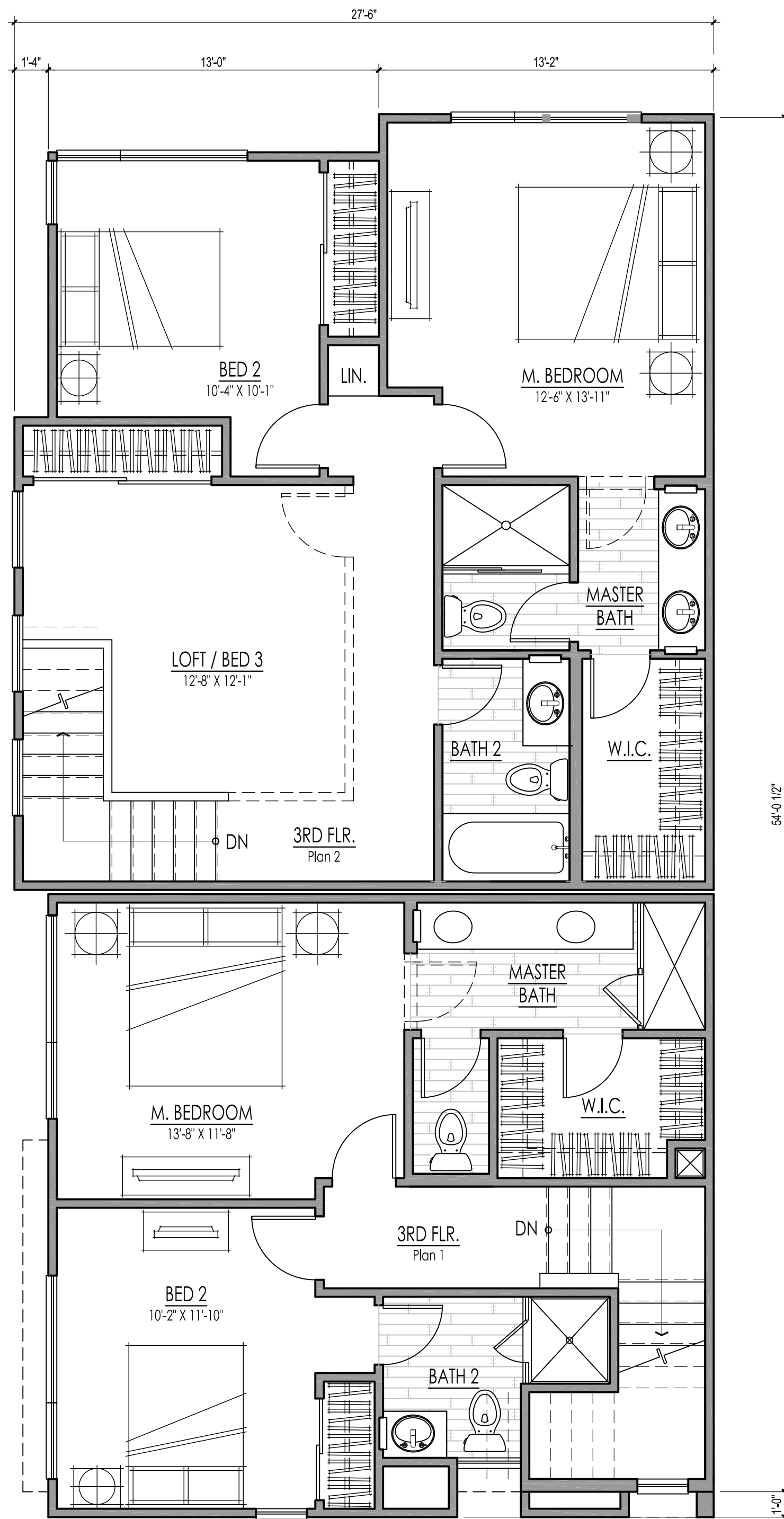
THIRD FLOOR
