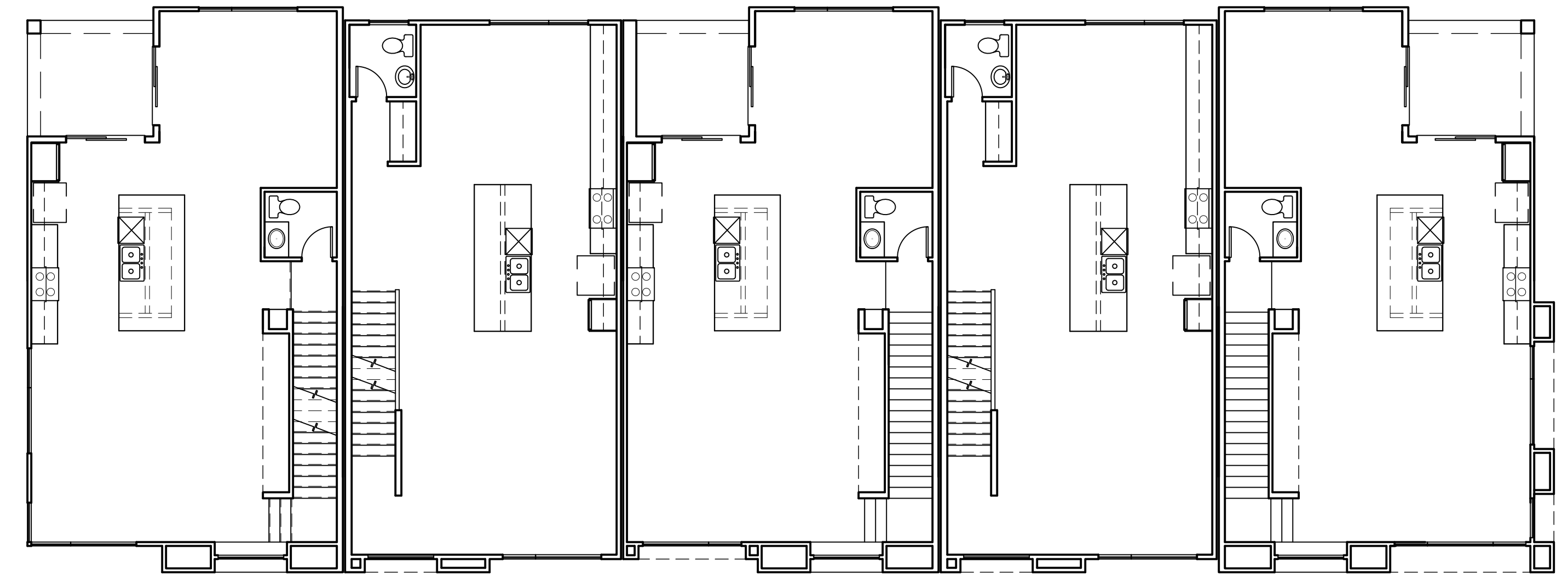
SECOND FLOOR
